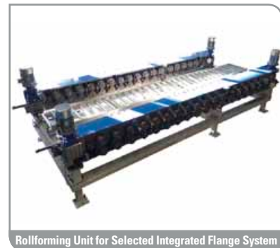
Rollforming Unit for Selected Integrated Flange System
