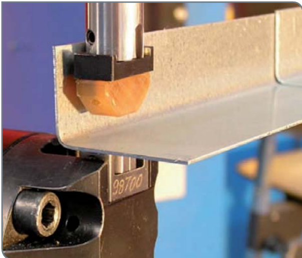
Rotating punch head for working on edges
